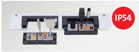
Rittal/Hoffman/Häwa Enclosure gland plates with slide frames for cable entry frames
